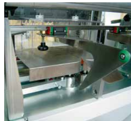
Adjustable Bag size. Movements on linear guides.
