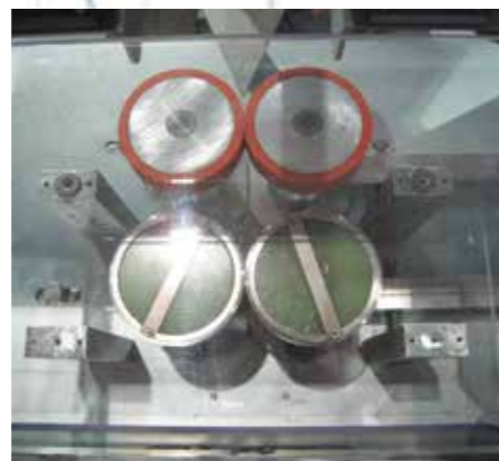
Sealing wheels and film tensioning .Rotary pulling and sealing wheels.
