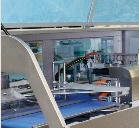
Packaging machine with side sealing to form the bag. Sealing.
