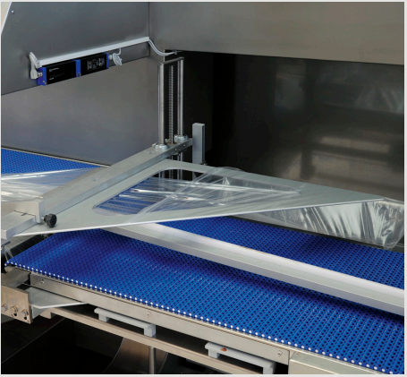
Film unwinding with triangle for flat film or mono-folding from reel. Rapid and simple format change without pre-formed bags. Highly versatile, with savings in material costs.
