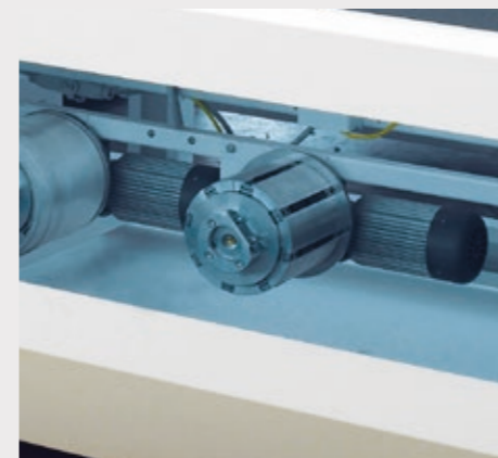
Double reel holder for box reels. Optional: handles on reel.
