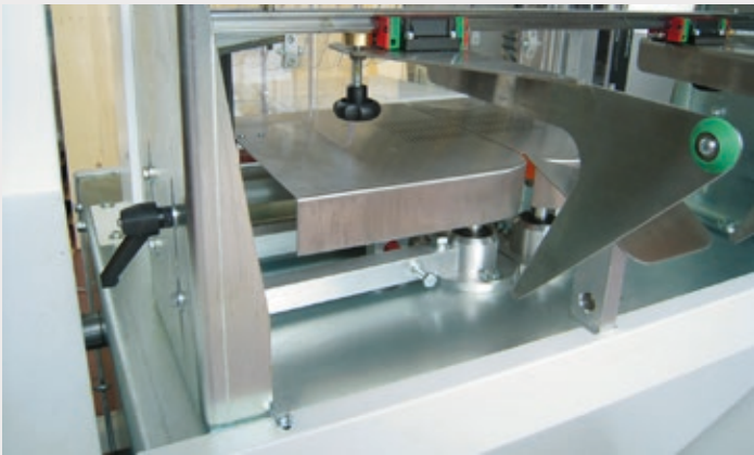
Adjustable bag measurement. All movements on linear guides.
