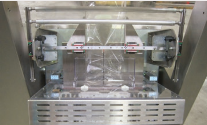
Tilting surface from 0° to 90° and precise product detecting through barrier electric eye
