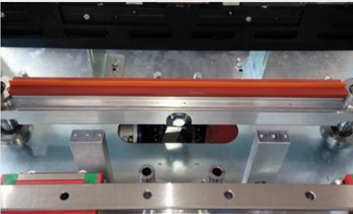
Motorised seal bar for use with PE and BOPP film.
