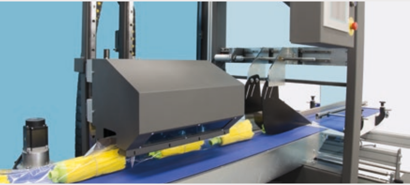
Built with the same structure and same philosophy, our Flowpack has the top or bottom sealer (reel from underneath or above) instead of the side reel.
