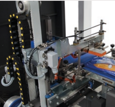
Motorized sealing bar with gusseting system.
