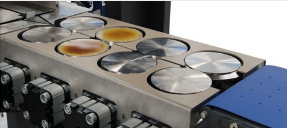
Four pairs of wheels, for sealing and fin folding. Wheels diameter min. 120 mm.
